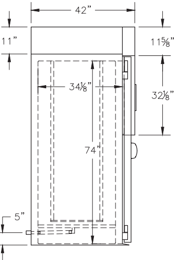
LATERAL VIEW
